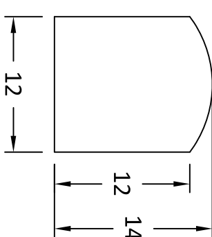
EXTENDED LEG SEGMENT SHAPE 60
