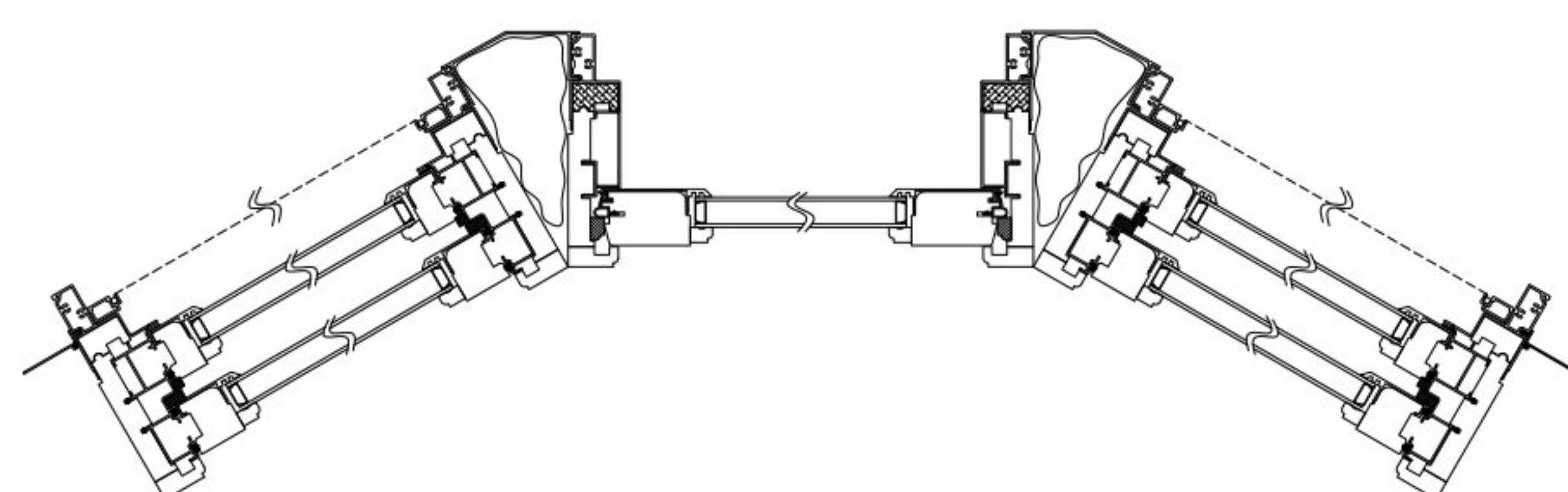
Double Hung Combination - 30° Bay Window
